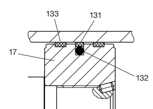
Low Friction Piston
